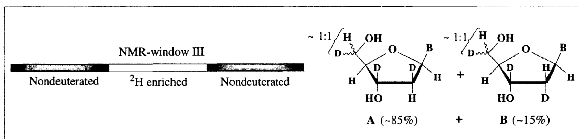
Figure 1. The "NMR-window III" concept (B = thymine-1-yl, cytosine-1-yl, adenine-9-yl or guanine-9-yl). For the "NMR-window I" and "NMR-window II" concepts, see refs 29 and 36.
