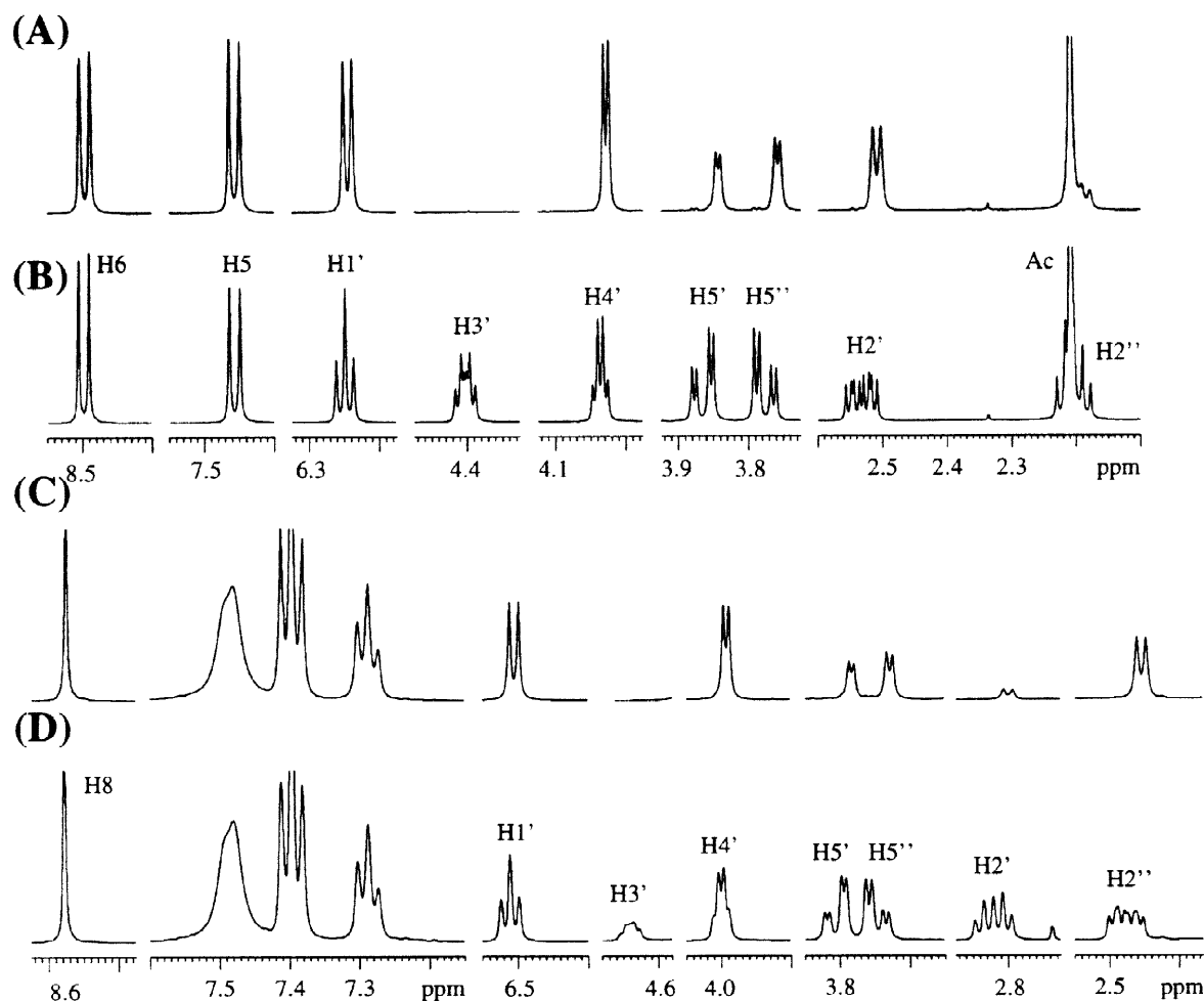
Figure 11: Aromatic and sugar regions of the 500 MHz ^1\text{H} -NMR spectra of deuterated- \beta -D-nucleosides and their natural-abundance counterparts: N^4 -acetyl-2'-deoxycytidine-2'-( R/S ),3',5'-( R/S )- ^2\text{H}_3 ( 50 ) (Panel A) and its natural-abundance counterpart (Panel B); N^2 -acetyl- O^6 -diphenylcarbamoyl-2'-deoxyguanosine-2'-( R/S ),3',5'-( R/S )- ^2\text{H}_3 ( 19 ) (Panel C) and its natural-abundance counterpart (Panel D).
