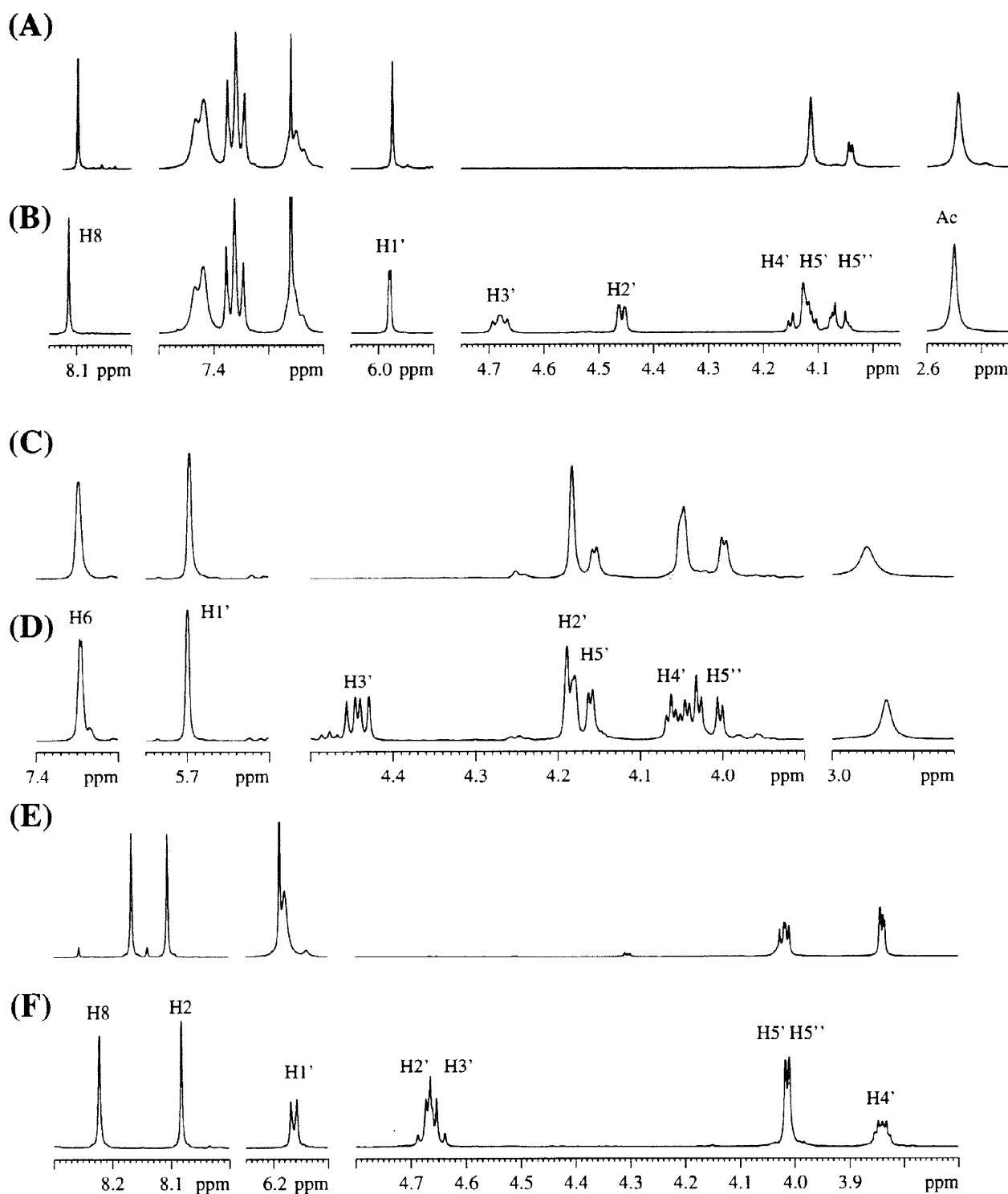
Figure 7: Aromatic and sugar regions of the 500 MHz ^1\text{H} -NMR spectra of deuterated- \beta - \underline{\text{D}} -nucleosides and their natural-abundance counterparts: 3',5'- O -TPDS- N 2 -acetyl- O 6 -diphenylcarbamoylguanosine-2',3',5'-( R/S )- ^2\text{H}_3 ( 16 ) (Panel A) and its natural-abundance counterpart (Panel B); 1-(3',5'- O -TPDS- \beta - \underline{\text{D}} -ribofuranosyl-3',5'-( R/S )- ^2\text{H}_2 )-thymine ( 30 ) (Panel C) and its natural-abundance counterpart (Panel D); 9-(3',5'- O -TPDS- \beta - \underline{\text{D}} -arabinofuranosyl-3',5'-( R/S )- ^2\text{H}_3 )-adenine ( 34 ) (Panel E) and its natural-abundance counterpart (Panel F).
