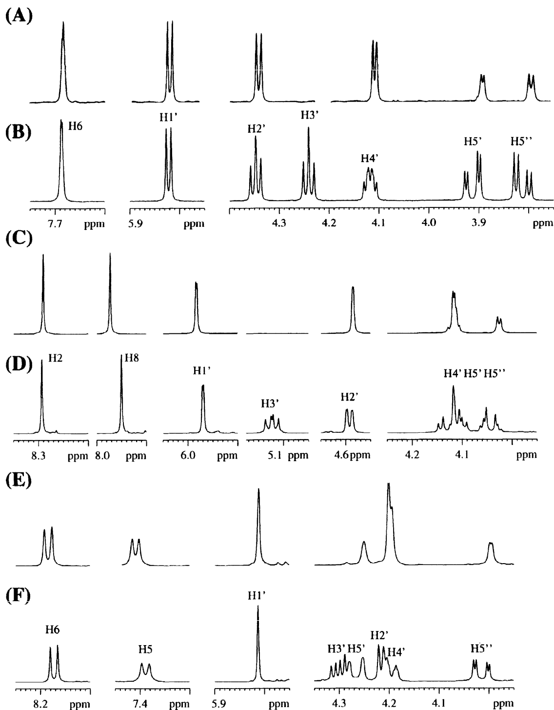
Figure 6: Aromatic and sugar regions of the 500 MHz ^1\text{H} -NMR spectra of deuterated- \beta -D-nucleosides and their natural-abundance counterparts: 1-( \beta -D-ribofuranosyl-3',5'-(R/S)- ^2\text{H}_2 )-thymine (26) (Panel A) and its natural-abundance counterpart (Panel B); 3',5'-O-TPDS-adenosine-3',5'-(R/S)- ^2\text{H}_2 (31) (Panel C) and its natural-abundance counterpart (Panel D); 3',5'-O-TPDS- N^4 -acetylcytidine-3',5'-(R/S)- ^2\text{H}_2 (32) (Panel E) and its natural-abundance counterpart (Panel F).
