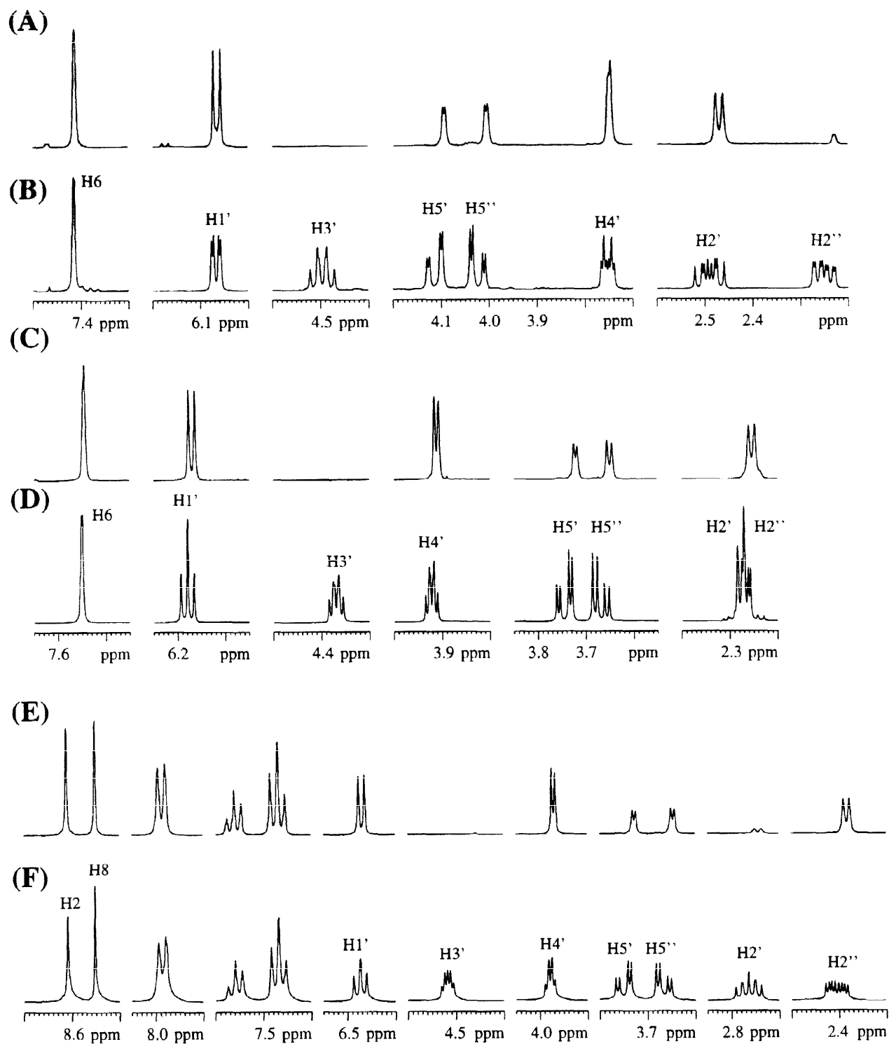
Figure 10: Aromatic and sugar regions of the 500 MHz ^1\text{H} -NMR spectra of deuterated- \beta - D -nucleosides and their natural-abundance counterparts: 3',5'- O -TPDS-thymidine-2'( R/S ),3',5'( R/S )- ^2\text{H}_3 (44) (Panel A) and its natural-abundance counterpart (Panel B); thymidine-2'( R/S ),3',5'( R/S )- ^2\text{H}_3 (48) (Panel C) and its natural-abundance counterpart (Panel D); N 6 -benzoyl-2'-deoxyadenosine-2'( R/S ),3',5'( R/S )- ^2\text{H}_3 (49) (Panel E) and its natural-abundance counterpart (Panel F).
