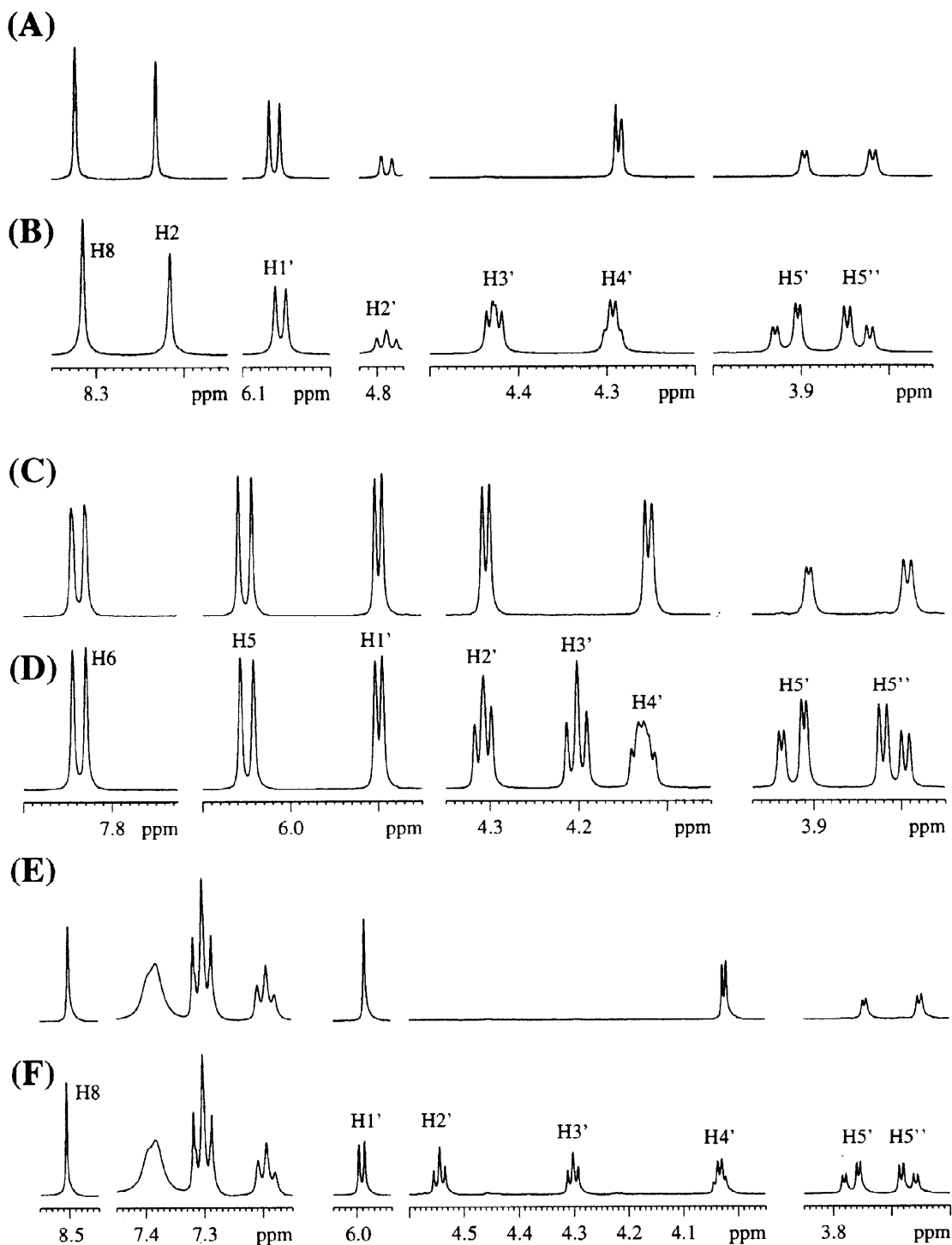
Figure 4: Aromatic and sugar regions of the 500 MHz ^1\text{H} -NMR spectra of deuterated- \beta -D-nucleosides and their natural-abundance counterparts: adenosine-3',5'-( R/S )- ^2\text{H}_2 (27) (Panel A) and its natural-abundance counterpart (Panel B); N 4 -acetylcytidine-3',5'-( R/S )- ^2\text{H}_2 (29) (Panel C) and its natural-abundance counterpart (Panel D); N 2 -acetyl- O 6 -diphenylcarbamoylguanosine-2',3',5'-( R/S )- ^2\text{H}_3 (15) (Panel E) and its natural-abundance counterpart (Panel F).
