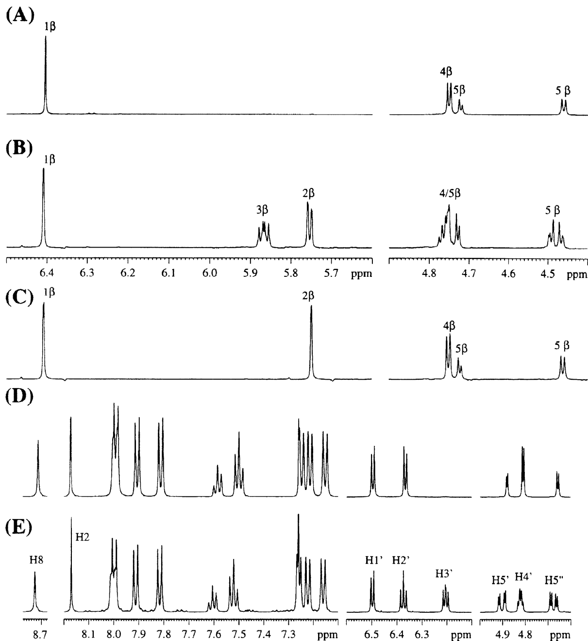
Figure 2: The sugar region of the 500 MHz ^1\text{H} -NMR spectra of 1- O -acetyl-2,3,5-tri- O -(4-toluoyl)- \beta - \underline{\underline{\text{D}}} -ribofuranose-2,3,5( \underline{\text{R}}/\underline{\text{S}} )- ^2\text{H}_3 ( 13 ) (Panel A), its natural-abundance counterpart (Panel B) and 1- O -acetyl-2,3,5-tri- O -(4-toluoyl)- \beta - \underline{\underline{\text{D}}} -ribofuranose-3,5( \underline{\text{R}}/\underline{\text{S}} )- ^2\text{H}_2 ( 22 ) (Panel C). The aromatic and sugar regions of the 500 MHz ^1\text{H} -NMR spectra of 2',3',5'- O -tri-(4-toluoyl)- N 6 -benzoyladenine-3',5'( \underline{\text{R}}/\underline{\text{S}} )- ^2\text{H}_2 ( 24 ) (Panel D) and its natural-abundance counterpart (Panel E).
