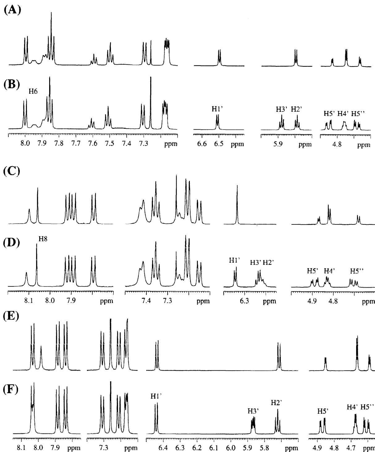
Figure 3: Aromatic and sugar regions of the 500 MHz ^1\text{H} -NMR spectra of deuterated- \beta -D-nucleoside derivatives and their natural-abundance counterparts: 2',3',5'- O -tri-(4-toluoyl)- N 4 -benzoylcytidine-3',5'-( R/S )- ^2\text{H}_2 ( 25 ) (Panel A) and its natural-abundance counterpart (Panel B); 2',3',5'- O -(4-toluoyl)- N 2 -acetyl- O 6 -diphenylcarbamoylguanosine-2',3',5'-( R/S )- ^2\text{H}_3 ( 14 ) (Panel C) and its natural-abundance counterpart (Panel D); 1-(2',3',5'-tri- O -(4-toluoyl)- \beta -D-ribofuranosyl)-thymine-3',5'-( R/S )- ^2\text{H}_2 ( 23 ) (Panel E); its natural-abundance counterpart (Panel F).
