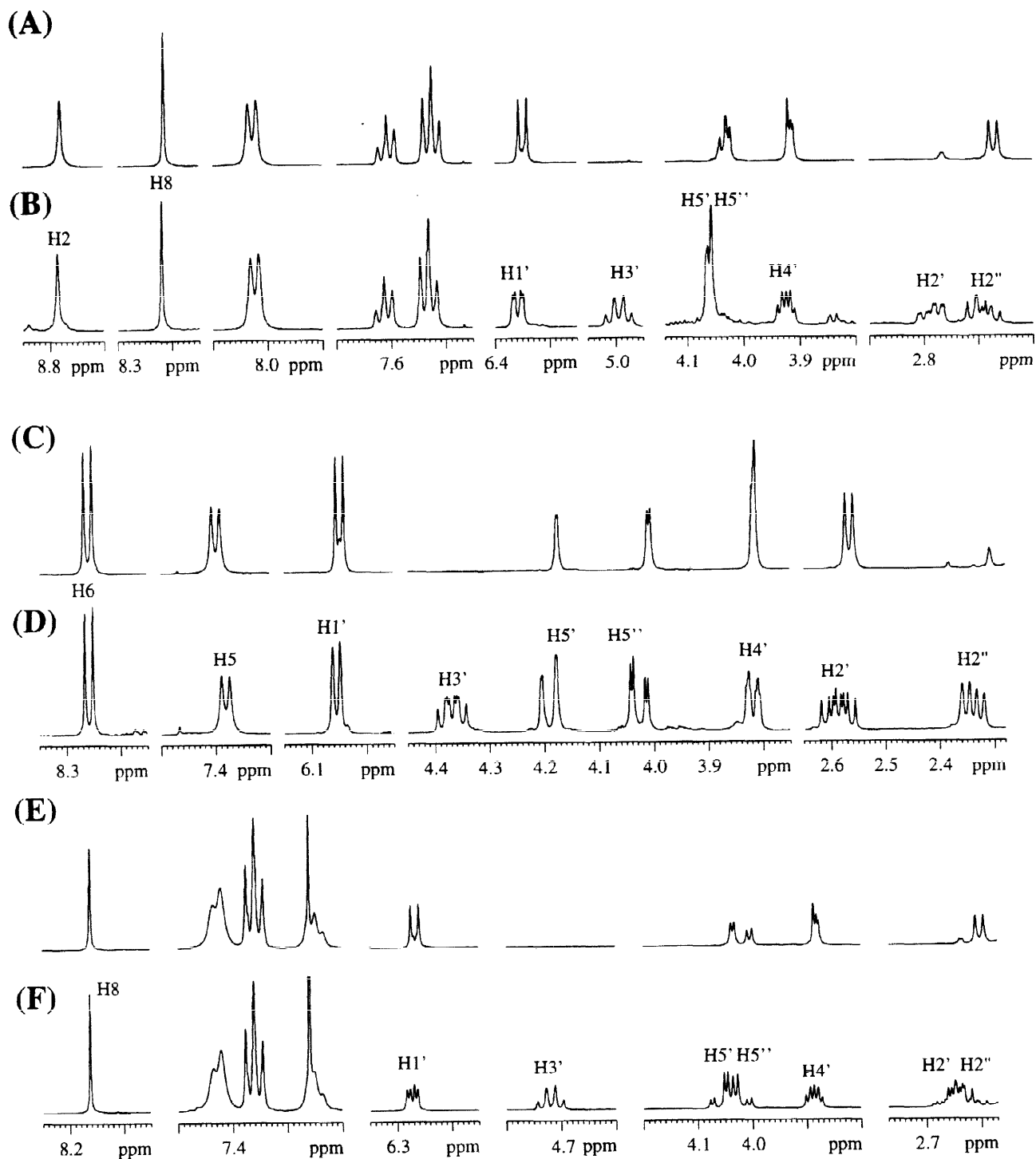
Figure 9: Aromatic and sugar regions of the 500 MHz ^1\text{H} -NMR spectra of deuterated- \beta -D-nucleosides and their natural-abundance counterparts: 3',5'-O-TPDS-2'-deoxyadenosine-2'-(R/S),3',5'-(R/S)- ^2\text{H}_3 (45) (Panel A) and its natural-abundance counterpart (Panel B); 3',5'-O-TPDS- N^4 -acetyl-2'-deoxycytidine-2'-(R/S),3',5'-(R/S)- ^2\text{H}_3 (46) (Panel C) and its natural-abundance counterpart (Panel D); 3',5'-O-TPDS- N^2 -acetyl- O^6 -diphenylcarbamoyl-2'-deoxyguanosine-2'-(R/S),3',5'-(R/S)- ^2\text{H}_3 (18) (Panel E) and its natural-abundance counterpart (Panel F).
