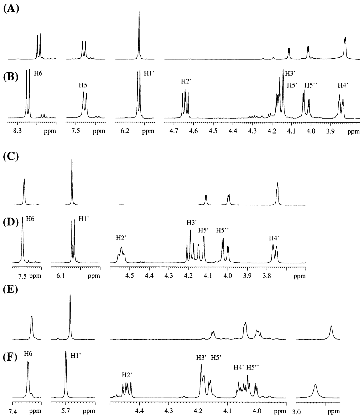
Figure 8: Aromatic and sugar regions of the 500 MHz ^1\text{H} -NMR spectra of deuterated- \beta -D-nucleosides and their natural-abundance counterparts: 1-(3',5'-O-TPDS- \beta -D-arabinofuranosyl-3',5'-(R/S)- ^2\text{H}_3 )- N^4 -acetylcytosine ( 35 ) (Panel A) and its natural-abundance counterpart (Panel B); 1-(3',5'-O-TPDS- \beta -D-arabinofuranosyl-3',5'-(R/S)- ^2\text{H}_3 )-thymine ( 33 ) (Panel C) and its natural-abundance counterpart (Panel D); 1-(3',5'-O-TPDS- \beta -D-ribofuranosyl-3',5'-(R/S)- ^2\text{H}_3 )-thymine ( 42 ) (Panel E) and its natural-abundance counterpart (Panel F).
